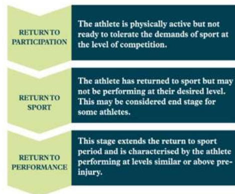
Figure 12. RTP Protocol
